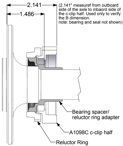
FIGURE # 1: Axle B-dimension
