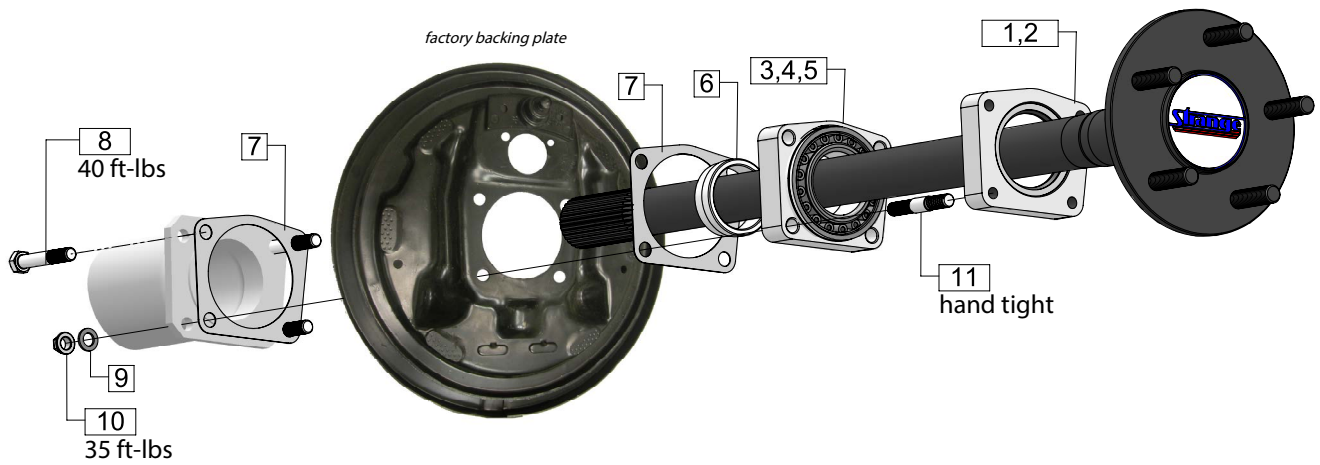
FIGURE # 2: Assembly
