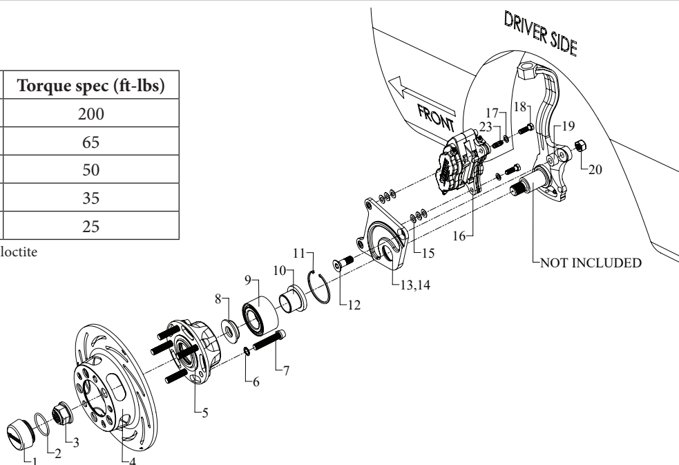
FIGURE # 2: Exploded B4184WC Assembly View
