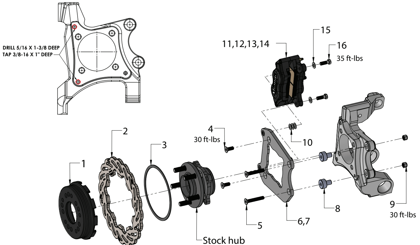
FIGURE # 2: B1723WCE Knuckle Modification
